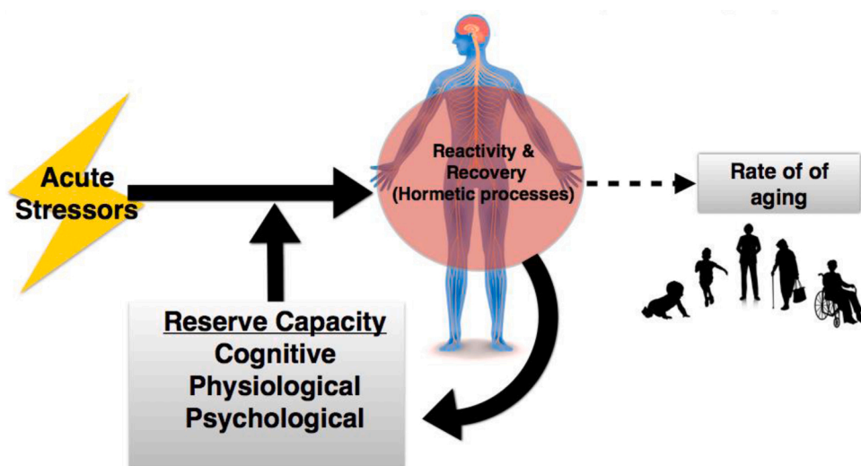
Fig. 2. Individual variance in acute stress response moderated by Reserve Capacity. In response to acute stressors, individuals have a kinetic trajectory of responses across psychological and physiological regulatory systems that lead to reactivity and recovery profiles. Resilient stress responses (typically rapid high peak and rapid recovery) often have hormetic effects at the cellular or systemic levels. High levels of reserve capacity predict more rapid recovery, and this may lead to a positive feedback loop promoting even higher reserve capacity. Level of stress resilience is multiply determined by the social context and individual reserve capacity. Together the latent homeostatic capacity of the organism to have resilient stress responses serves as an indicator of biological age and over time may influence the rate of aging.
